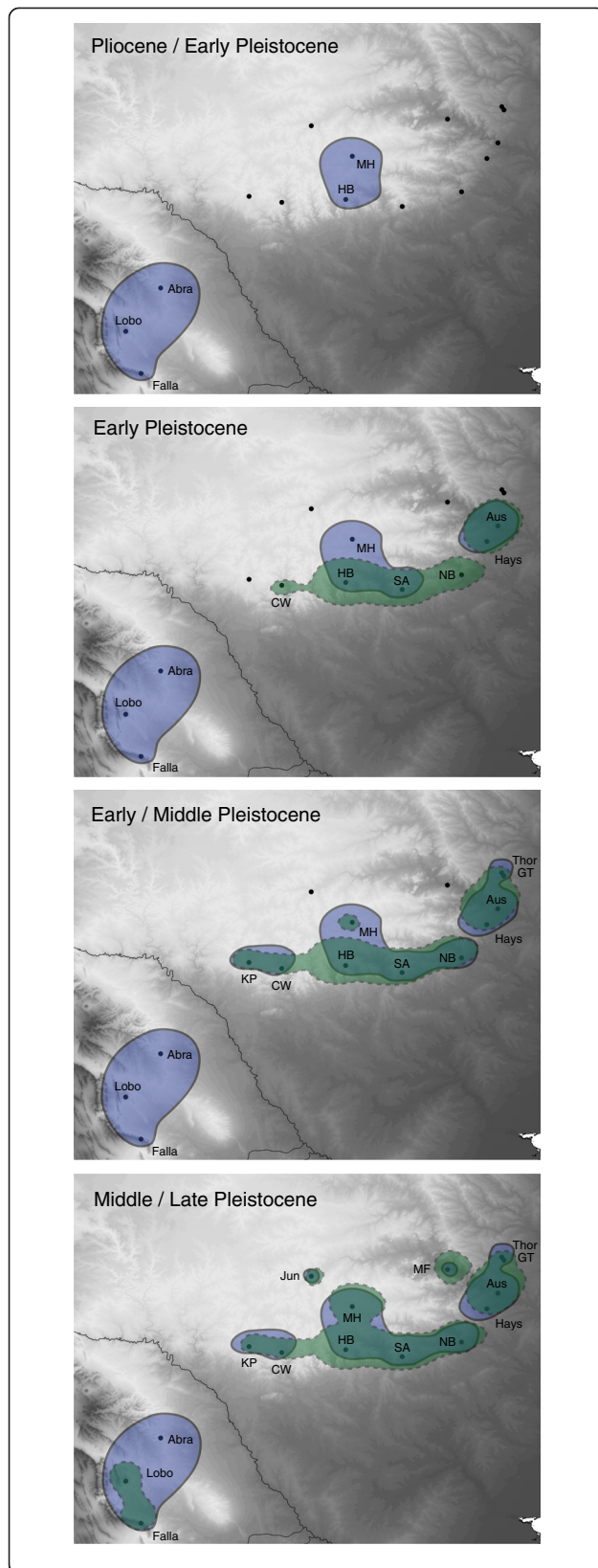
Figure 4 Reconstructions of the spatial history of the North American vaejovid scorpions Pseudouroctonus reddelli and Pseudouroctonus sprousei based on Bayesian analyses of mitochondrial DNA (solid line) and nuclear internal transcribed spacer region (ITS) data (dashed line). Polygons represent 80% highest posterior density intervals for the spatial location of ancestral populations across four time slices. Abbreviations for sampled localities in Table 3.
