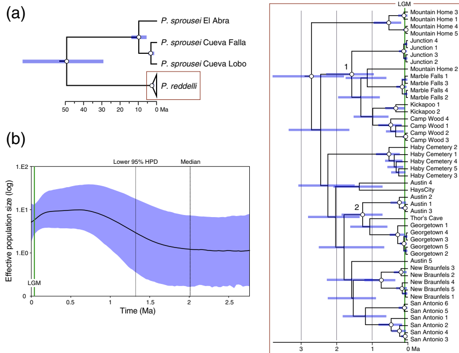
Figure 2 Phylogeographical structure and demographic reconstruction through time inferred from 1,152 base pairs of mitochondrial DNA for the North American vaejovid scorpions Pseudouroctonus reddelli and Pseudouroctonus sprousei . (a) Time-calibrated Bayesian gene tree for P. reddelli and P. sprousei . Nodes that received \geq 0.95 posterior probability support depicted with white dots. Two strongly supported subclades of P. reddelli are numbered (1 and 2). (b) Bayesian skyride plot for P. reddelli , showing change in effective population size of females since the time of the most recent common ancestor. HPD = highest posterior density; LGM = Last Glacial Maximum.
